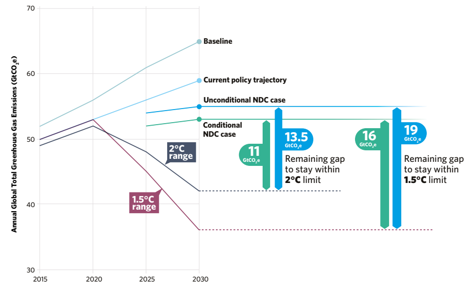
GLOBAL GREENHOUSE GAS EMISSIONS UNDER DIFFERENT SCENARIOS AND THE EMISSIONS GAP IN 2030
